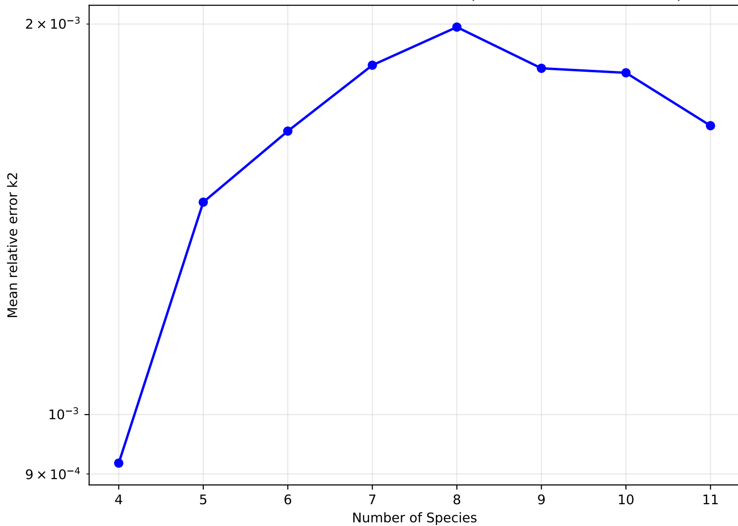
30, 30 — Mean relative error k2 vs number of species (zoomed: 4 to 11 species)
